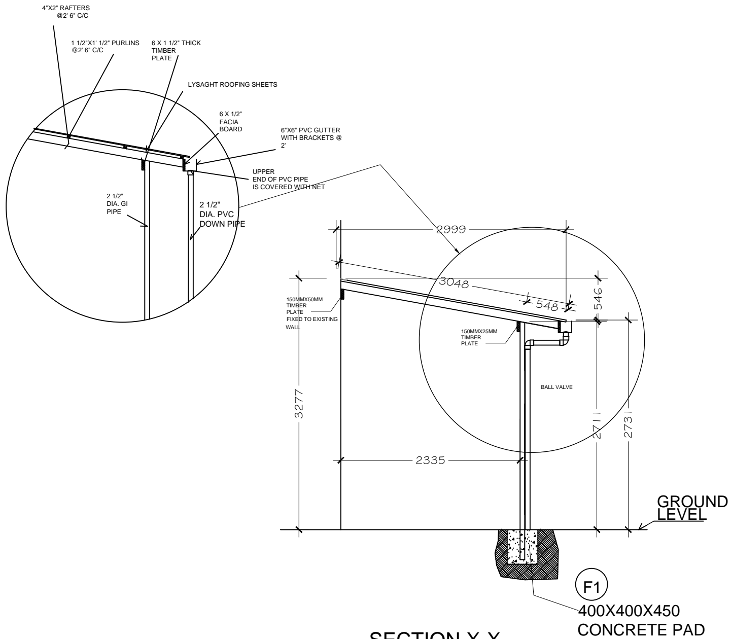
SECTION X-X 1:50
