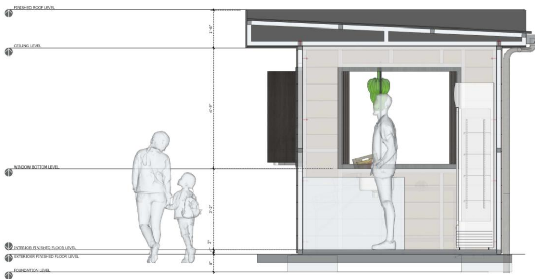
SECTION - X
