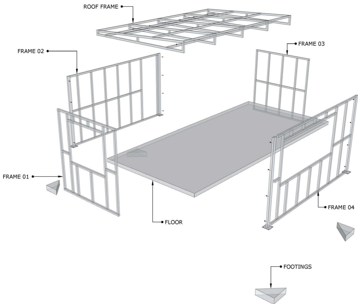
EXPLODED STRUCTURE VIEW
